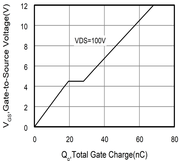
Figure 5. Gate Charge
