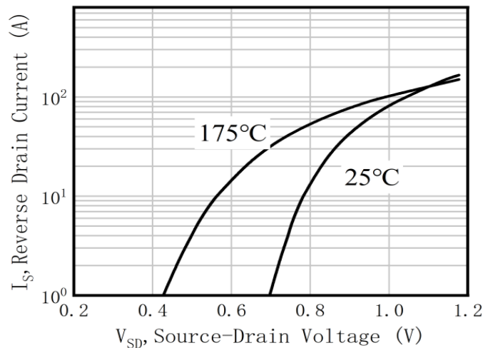
Figure 6. Body Diode Forward
