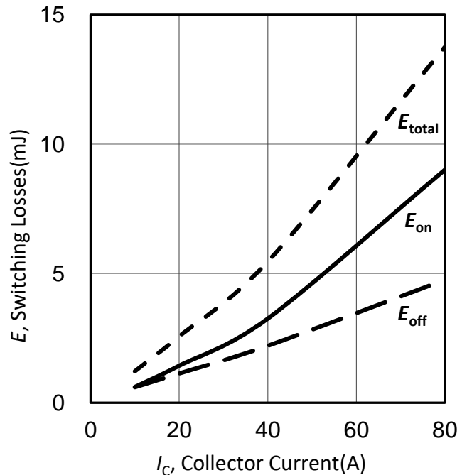
Figure 20. Typical switching times as a function of collector current (inductive load, T_{vj}=175^{\circ}\text{C} , V_{CE}=600\text{V} , V_{GE}=0/15\text{V} , R_G=10\Omega )
